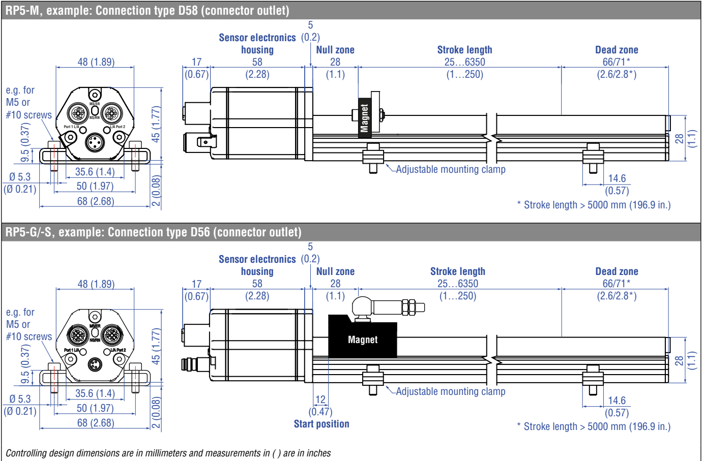
Fig. 3: Temposonics® RP5 with U-magnet/magnet slider
