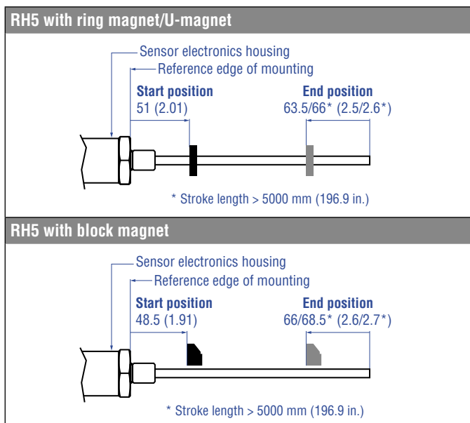
Fig. 35: Start- and end positions of magnets RH5
