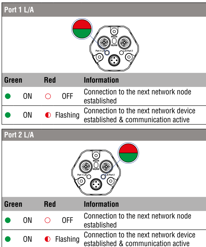
Fig. 52: LED status, part 2
