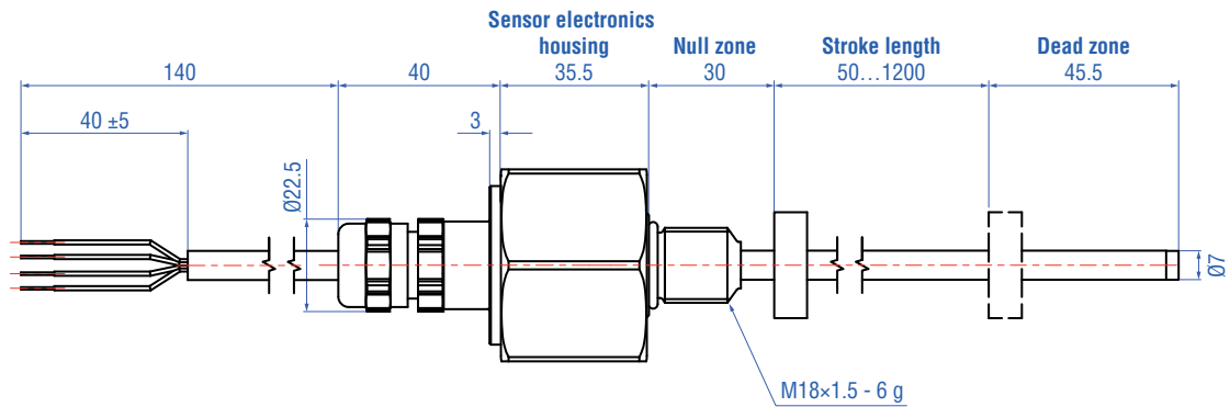
Fig. 7: Temposonics® MH-Series MH Threaded (MH-P)
